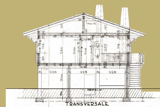
TRANSVERSALE
